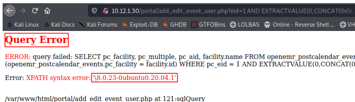
Figure 3.19: OpenEMR SQLi POC
